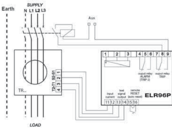
ELR96P - shunt trip wiring
