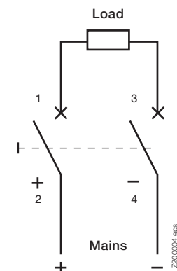
Connection diagram, two-pole (max. 250 V=) S402M-UCC
