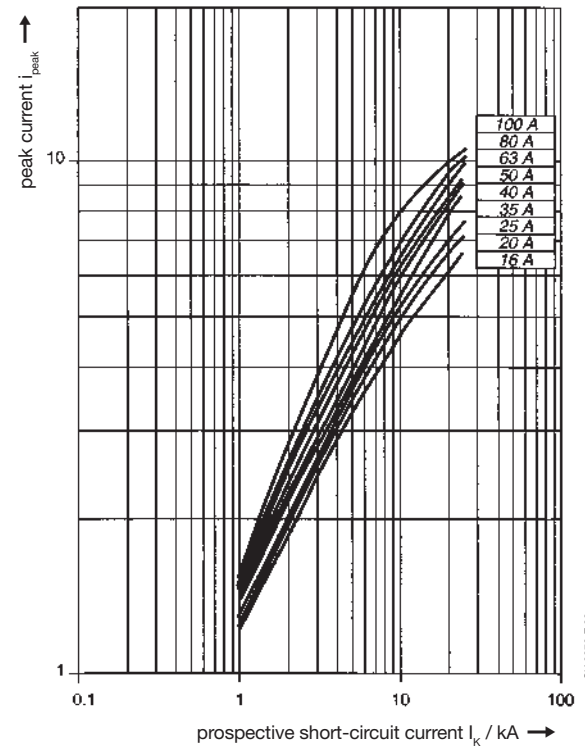
S 700 characteristic K selective let-through peak current ( I_{peak} )
