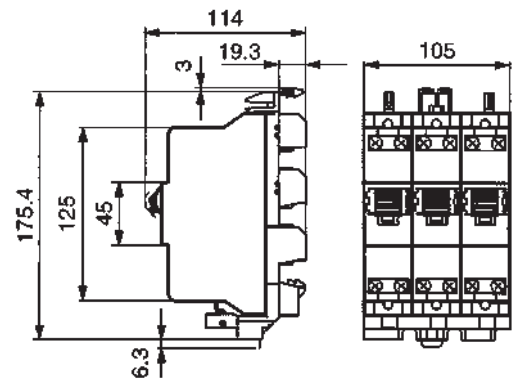
3 x S 701 with busbar adapter
