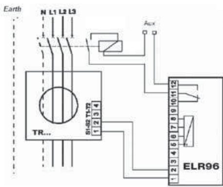
ELR96 - shunt trip wiring
