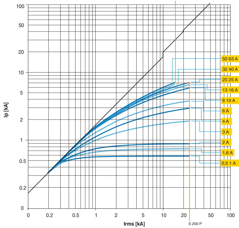
S 200-S 200 M-S 200 P, characteristic Z
