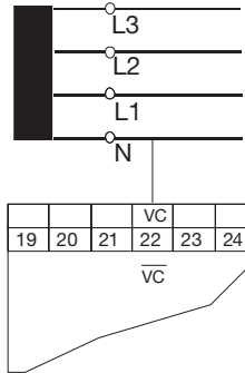
Three-phase network with neutral Max 1100V L-L
