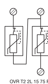
OVR T2 2L 15 75 P
