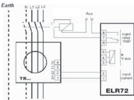
ELR72 - shunt trip wiring
