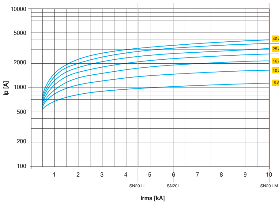
10 SN 201 L, SN 201, SN 201 M, characteristic B 230 V
