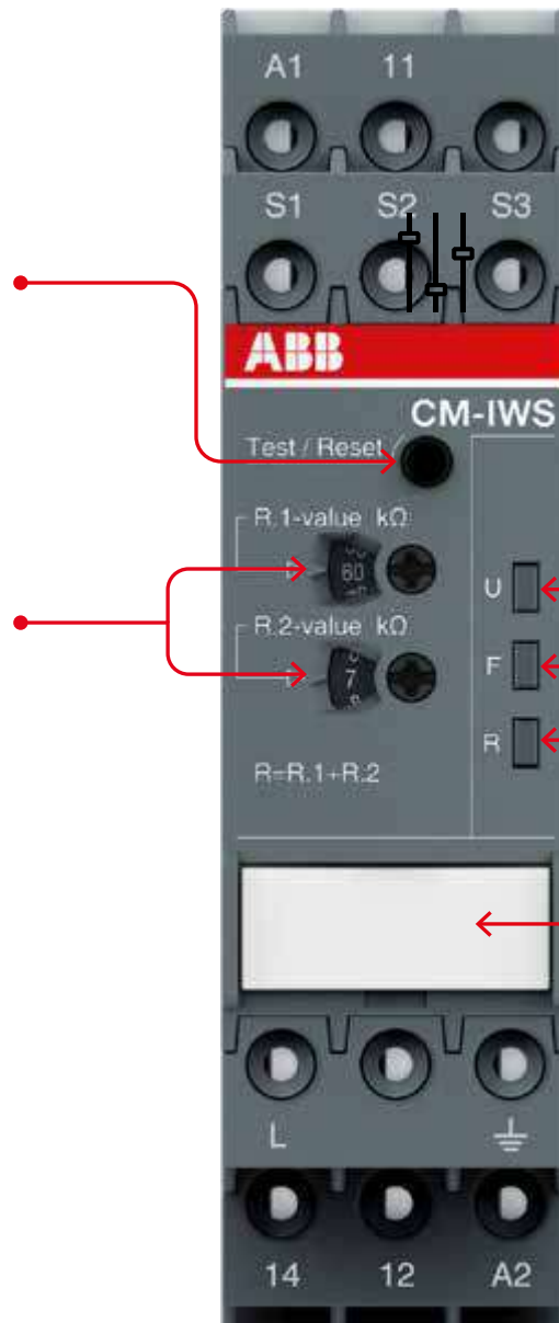
Configuration and setting Front-face rotary switches for threshold value adjustment:
