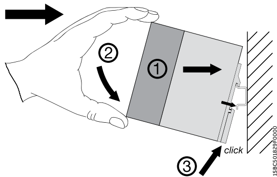
Mounting
