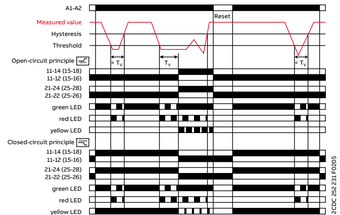
Undervoltage monitoring with latching
