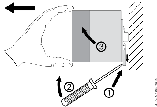
Dismounting
