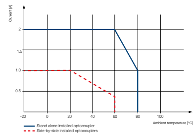
Derating curve Triac output CR-S
