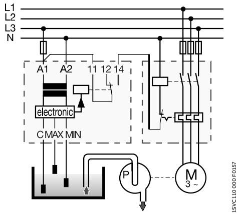
Liquid level control - drain
