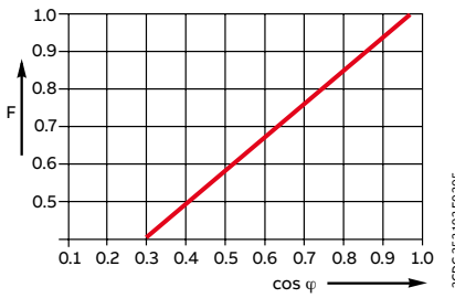
Derating factor F for inductive AC load
